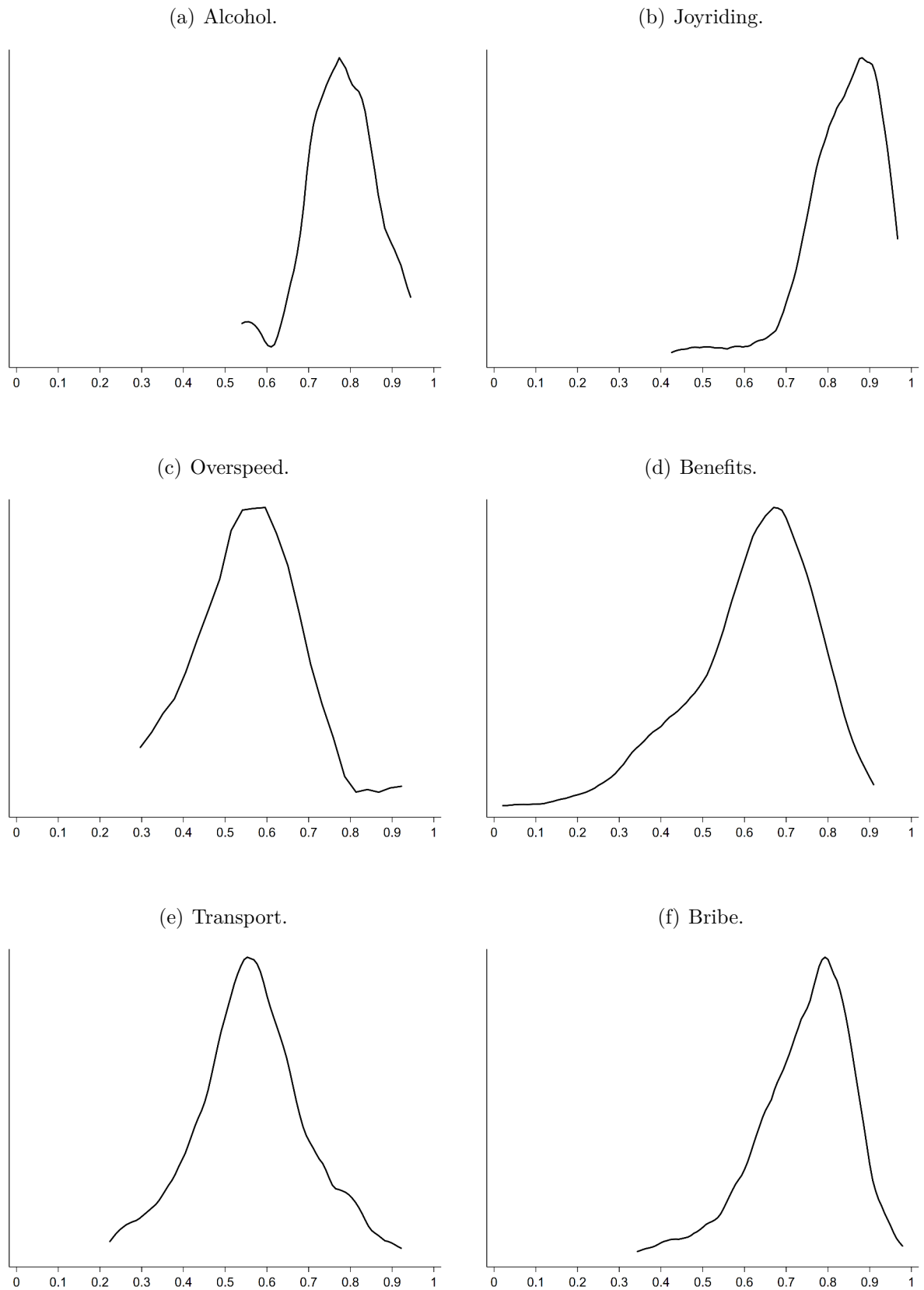
Figure A1: Distributions of norms of compliance.
